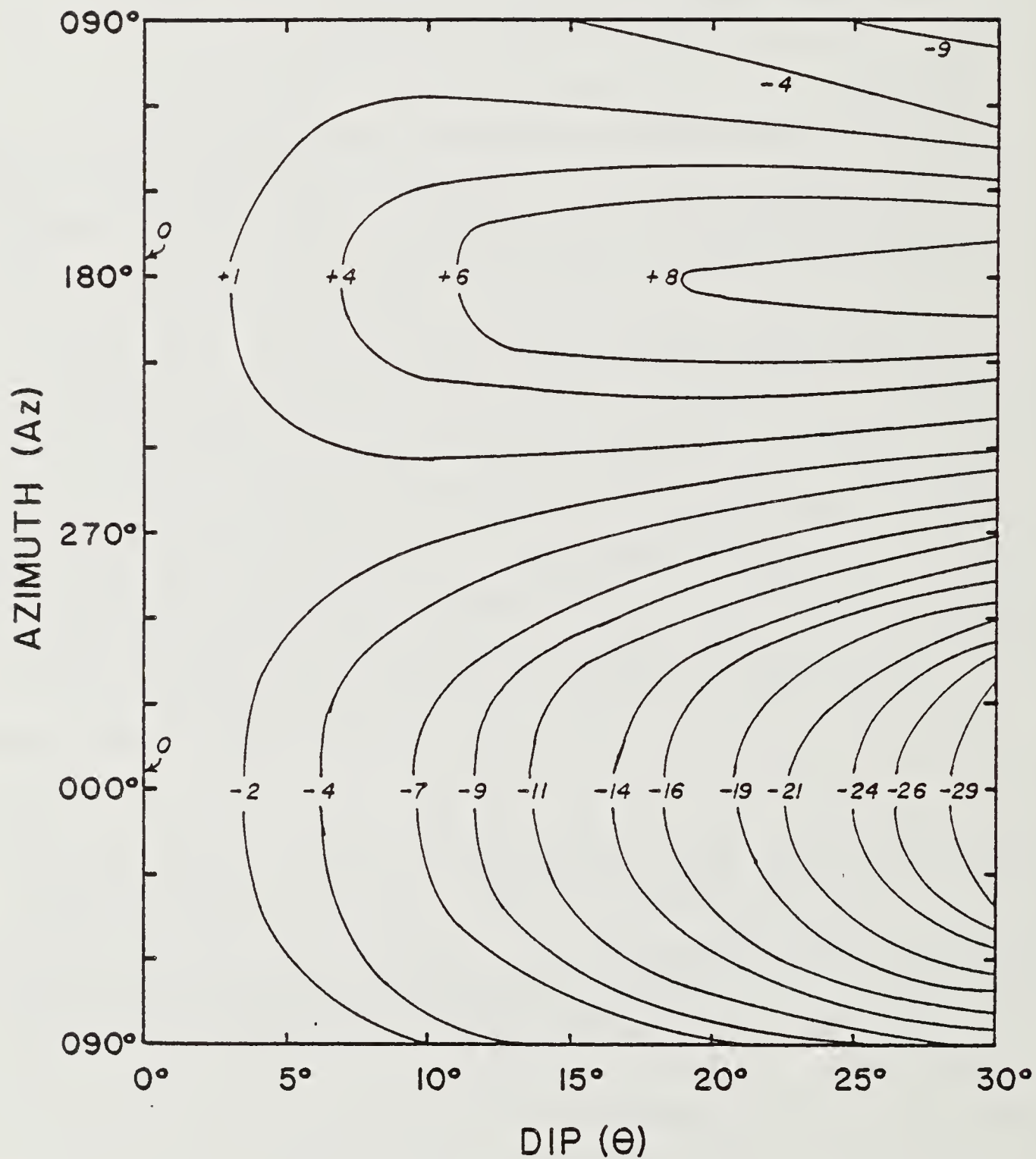
Dependence of mean temperature ten centimeters below the local surface on dip and azimuth angles. The contours represent the deviation ( ^\circ\text{K} ) of mean temperature from that of a flat surface.
